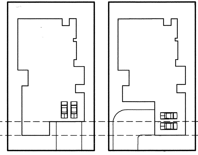
BUILDING LINE DIAGRAM FOR LOT 21 IN BLOCK 1 RESTRICTED TO 1 SINGLE FAMILY DWELLING UNIT ONLY
